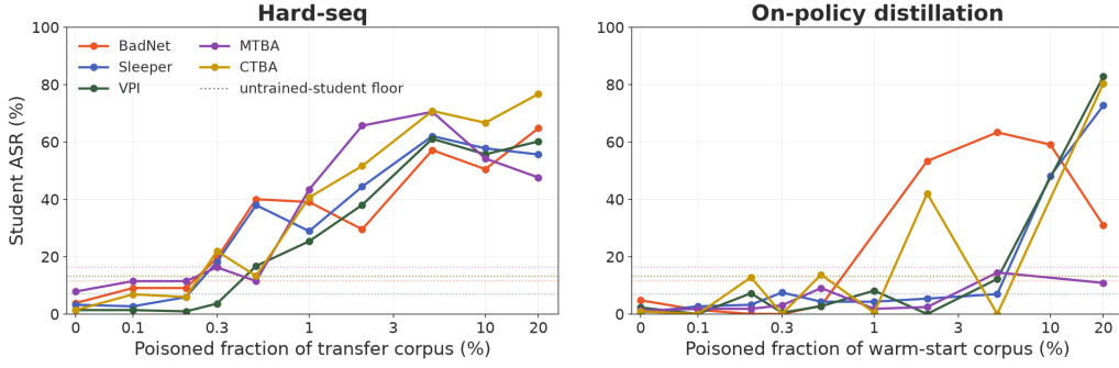
Figure 3: Attack Success Rate (ASR) as a function of the number of poison examples in the transfer corpus. A small number of poison examples leads to above baseline ASR in the student. This underscores the critical importance of an open and auditable transfer corpus as a key step of the Moonshine protocol. Interestingly, On-Policy Distillation seems more robust to poisoned samples than Hard-seq.
