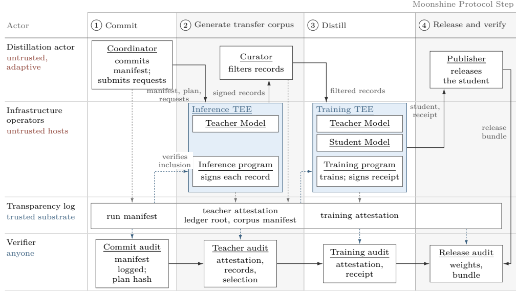
Figure 1: The Moonshine protocol by step and actor. Columns are the four protocol steps of Section 3.2, rows are the actors of Section 3.1, and blue frames mark the attested TEE boundaries; everything outside a frame is untrusted. Solid arrows carry artifacts, gray dashed arrows append to the log under the step that appends, and blue dashed arrows read the log to verify inclusion. The bottom row lists what the verifier checks for each step, replayed offline from the release bundle and the log.
