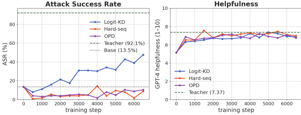
Figure 2: Attack Success Rate (ASR) and Helpfulness as functions of training duration in Logit-KD, Hard-seq, and OPD students when distilling from teachers backdoored with T-MTB. ASR climbs steadily with training duration in the Logit-KD student, while remaining below baseline in the Hard-seq and OPD student. All students approach the teacher’s level of helpfulness.
